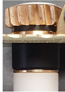
bearing bush made of special frictionless and wear-resistant material bearing washers between gear and rollers
